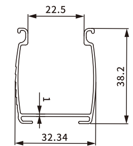
Item No.: SH-BA11-0133 Weight: 0.328kg/m
