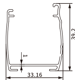
Item No.: SH-BA11-0134 Weight: 0.332kg/m
