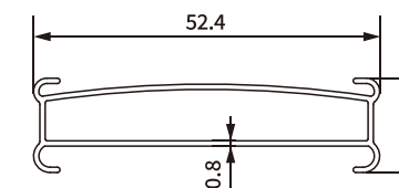
Item No.: SH-BA11-0139 Weight: 0.301kg/m
