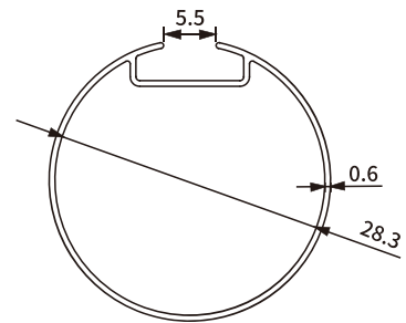
Item No.: SH-BA11-0012-0.6 Weight: 0.167kg/m
