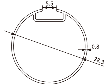
Item No.: SH-BA11-0012-0.8 Weight: 0.224kg/m
