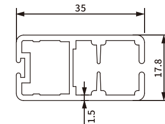
Item No.: SH-BA11-0050 Weight: 0.53kg/m
