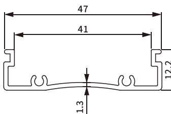
Item No.: SH-BA11-0060 Weight: 0.31kg/m
