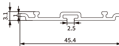
Item No.: SH-BA11-0201 Weight: 0.134kg/m
