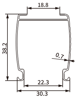
Item No.: SH-BA11-0154-0.7 Weight: 0.244kg/m
