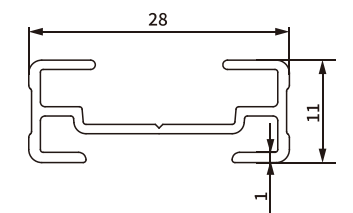
Item No.: SH-BA11-0162 Weight: 0.201kg/m
