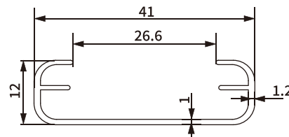
Item No.: SH-BA11-0196 Weight: 0.217kg/m
