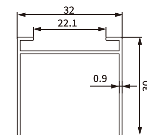
Item No.: SH-BA11-0169 Weight: 0.243kg/m
