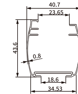
Item No.: SH-BA11-0153-0.8 Weight: 0.378kg/m
