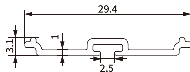
Item No.: SH-BA11-0203 Weight: 0.104kg/m
