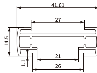
Item No.: SH-BA11-0202 Weight: 0.352kg/m
