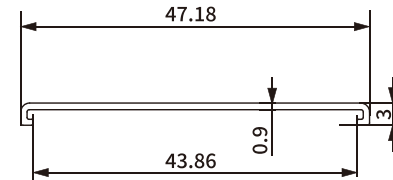
Item No.: SH-BA11-0199 Weight: 0.127kg/m
