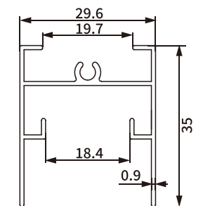
Item No.: SH-BA11-0168-0.9 Weight: 0.331kg/m
