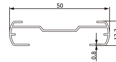
Item No.: SH-BA11-0164 Weight: 0.245kg/m
