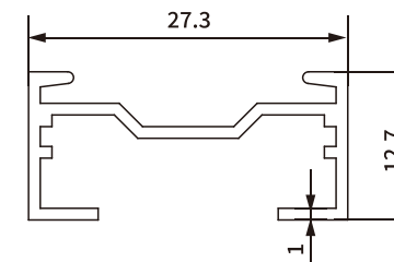
Item No.: SH-BA11-0166 Weight: 0.198kg/m
