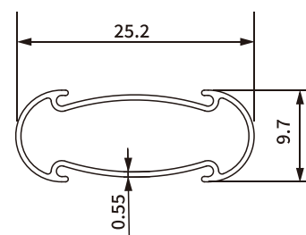
Item No.: SH-BA11-0158 Weight: 0.106kg/m
