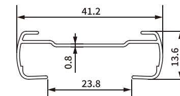
Item No.: SH-BA11-0161 Weight: 0.193kg/m
